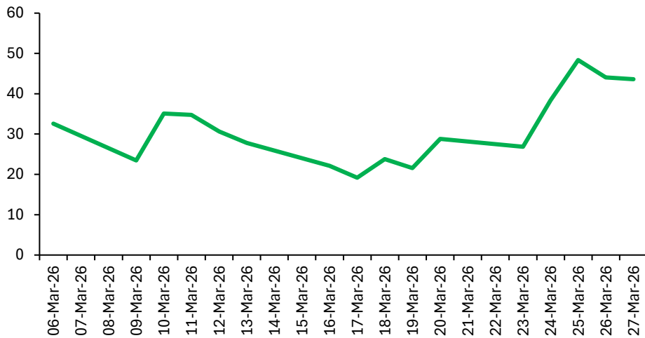
RSI Movement
